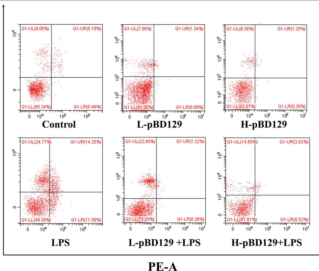
FIGURE 4 | Percentage of apoptotic cells in the jejunal mucosal of mouse. Frames were divided into four quadrants: Q1–UL represents necrotic cells. Q1–UR represents late-stage apoptotic cells. Q1–LL represents normal cells. Q1–LR represents early-stage apoptotic cells. Control, 200 \mu L sterile saline; LPS, 200 \mu L Lipopolysaccharide; L-pBD129, 200 \mu L of 0.6 mg/ml porcine \beta -defensin; H-pBD129, 200 \mu L of 1.2 mg/mL porcine \beta -defensin 129; L-pBD129 + LPS, 200 \mu L of 0.6 mg/mL pBD129 pretreated followed by LPS treated; H-pBD129 + LPS, 200 \mu L of 1.2 mg/mL pBD129 pretreated followed by LPS treated. n = 3 /group.
