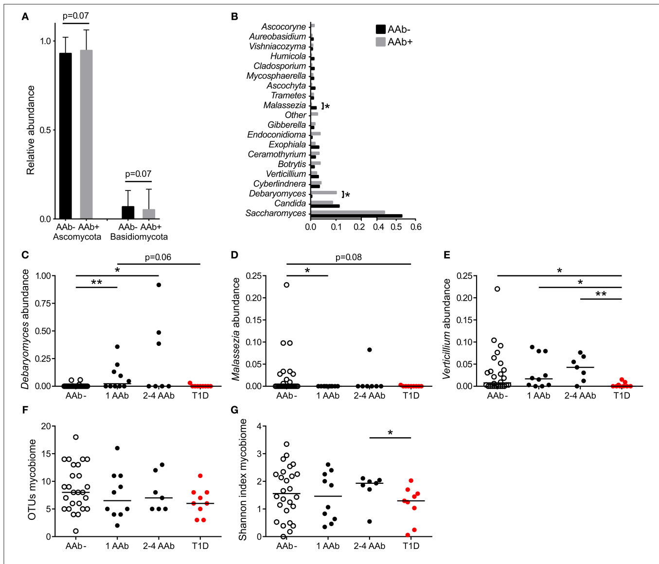
FIGURE 2 | Fungal community characteristics in children with or without T1D-associated autoantibodies. (A) Relative abundance of fungal phyla Ascomycota (left columns) and Basidiomycota (right columns). Children without autoantibodies: black columns and children with autoantibodies: gray columns. (B) Relative abundance of 20 most abundant fungal genera in children with (gray bars) and without autoantibodies (black bars). (C–E) The relative abundances of Debaryomyces (C) , Malassezia (D) , and Verticillium (E) in healthy children without autoantibodies, in children with a different number of autoantibodies and in children who have progressed from autoantibody-positive state to clinical T1D. (F,G) Number of OTUs and Shannon diversity index in healthy children without autoantibodies, in children with a different number of autoantibodies and in children who have progressed from autoantibody-positive state to clinical T1D. Healthy children without autoantibodies are marked with open circles, children with 1–4 autoantibodies with black circles and children who have progressed to clinical disease with red circle. p -values were calculated with the Mann–Whitney U -test. * p < 0.05, ** p < 0.01.
